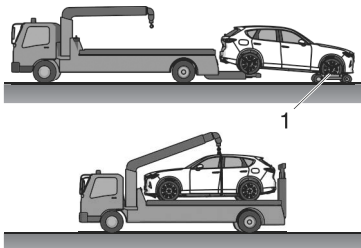
1 Wheel dollies
